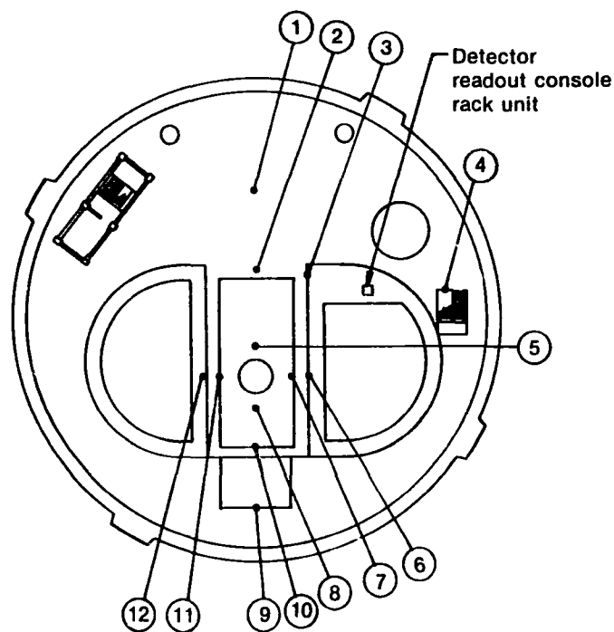
Reactor building 347-ft elevation
