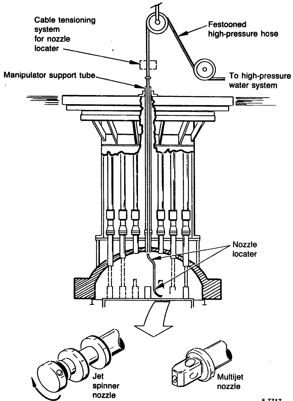
Figure A-20. Plenum plate flushing concept.
