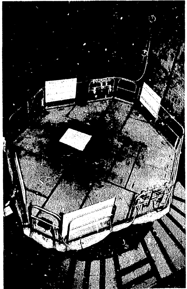
Figure 26. IIF installed on reactor vessel flange.
