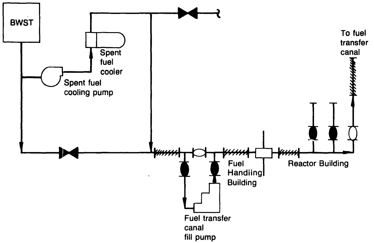
Figure A-4. Fuel transfer canal fill system.
