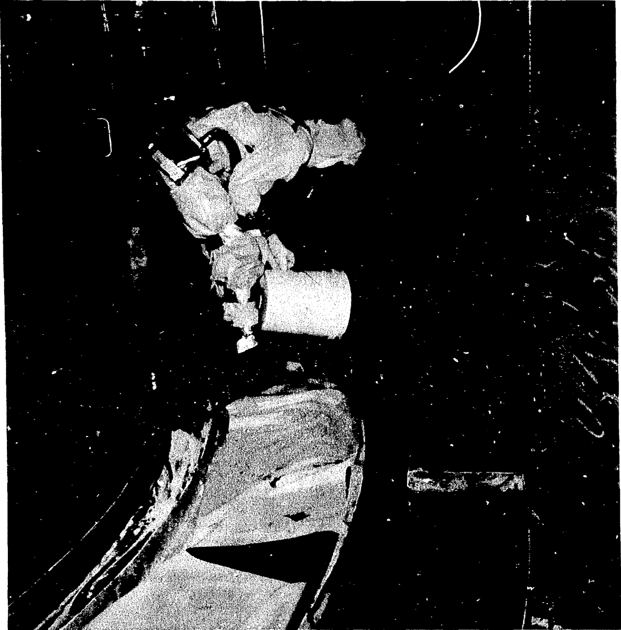
Figure 11. Canal seal plate—pouring sealant in barrier angles.
