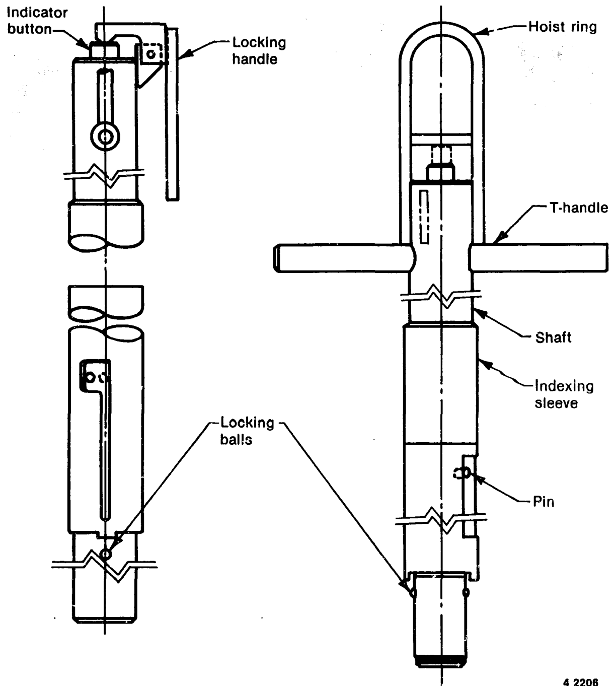
Figure 13. Lead screw lifting tool.
