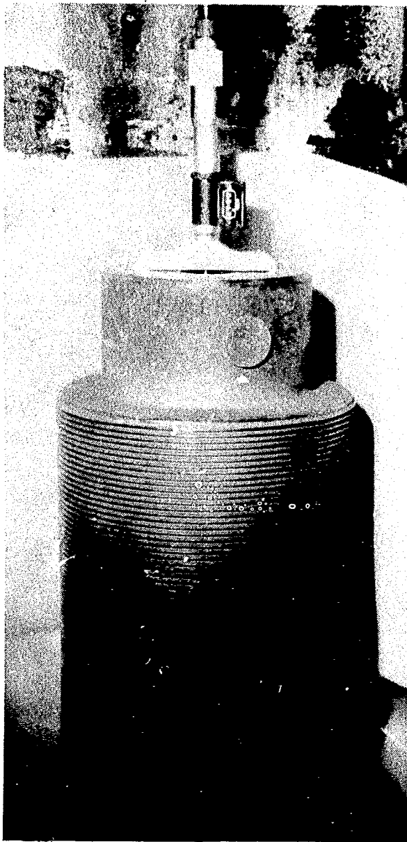
Figure 19. Stud elongation measuring tool (depth micrometer).
