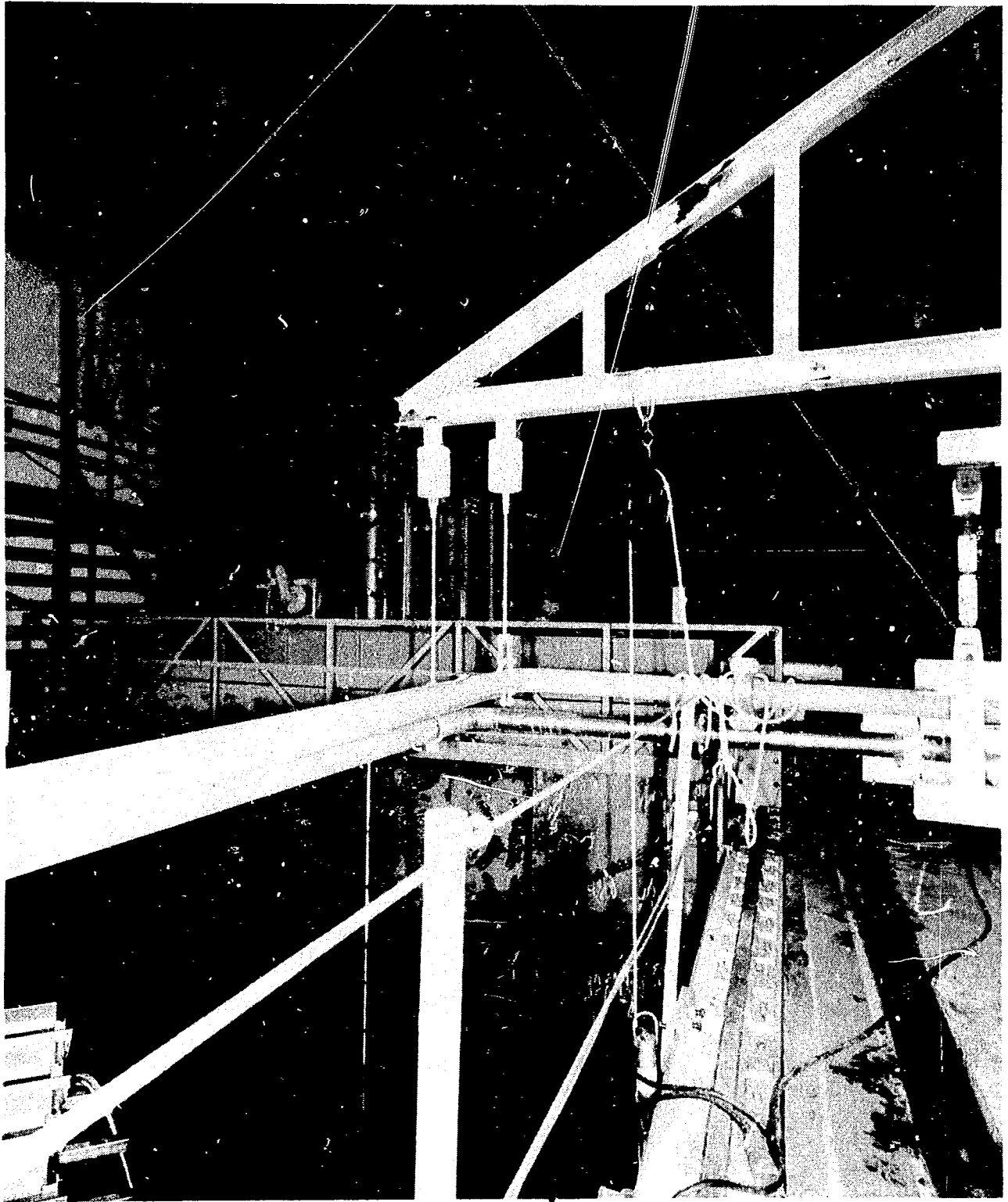
Figure 8. Cooling water spool piece and support hanger.
