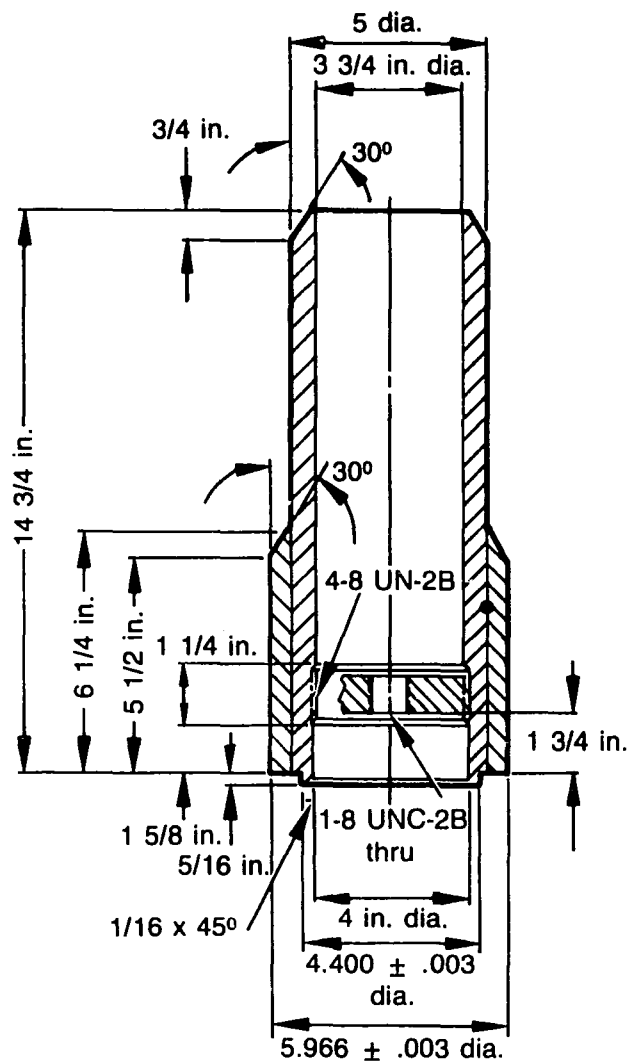
Figure A-16. Modified guide stud assembly.
