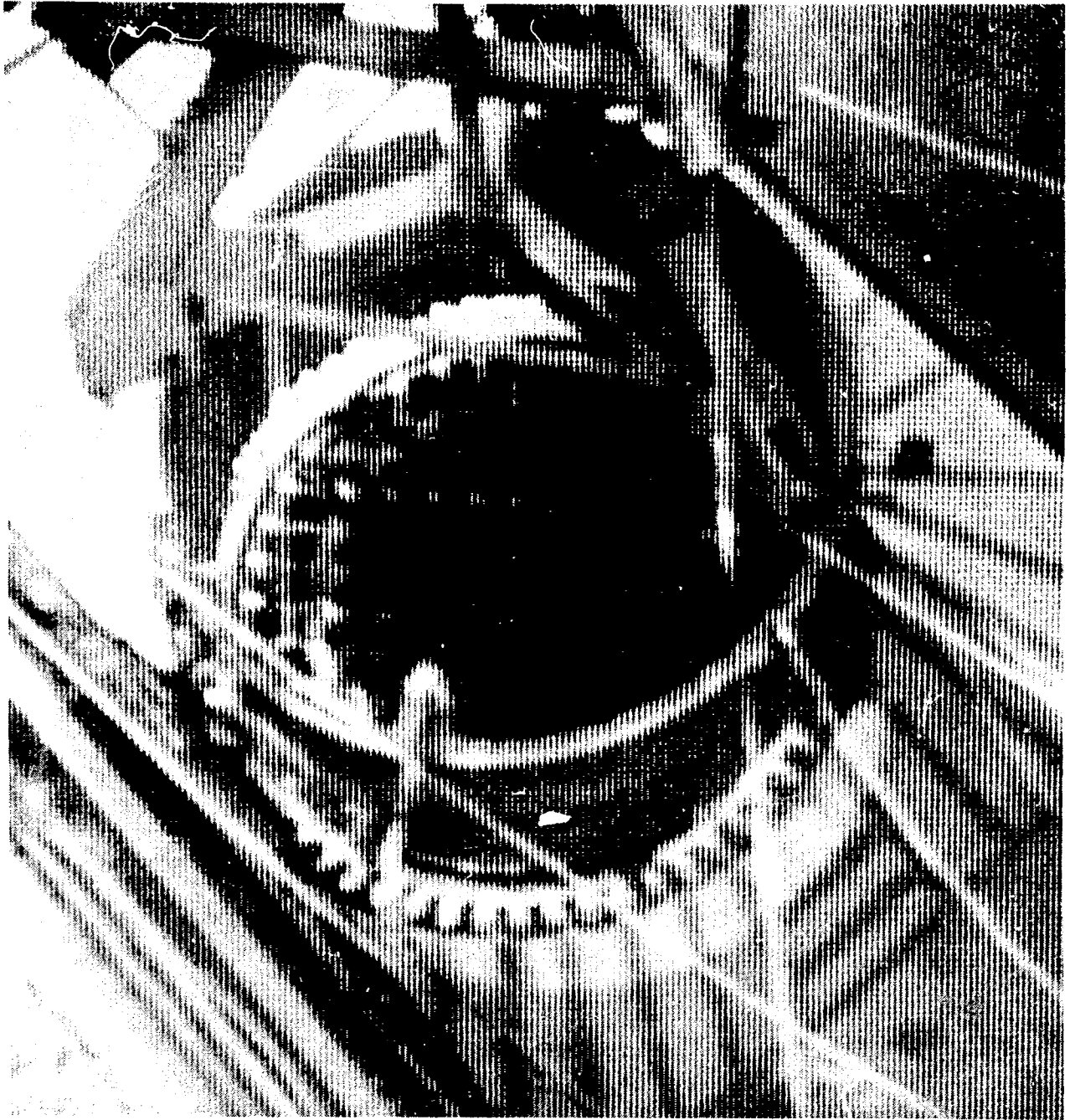
Figure 32. IIF lowered onto the reactor vessel flange.
