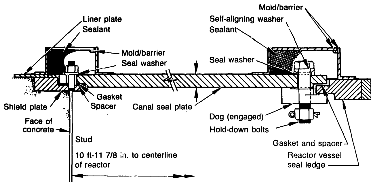
Figure A-9. Canal seal plate modifications.
