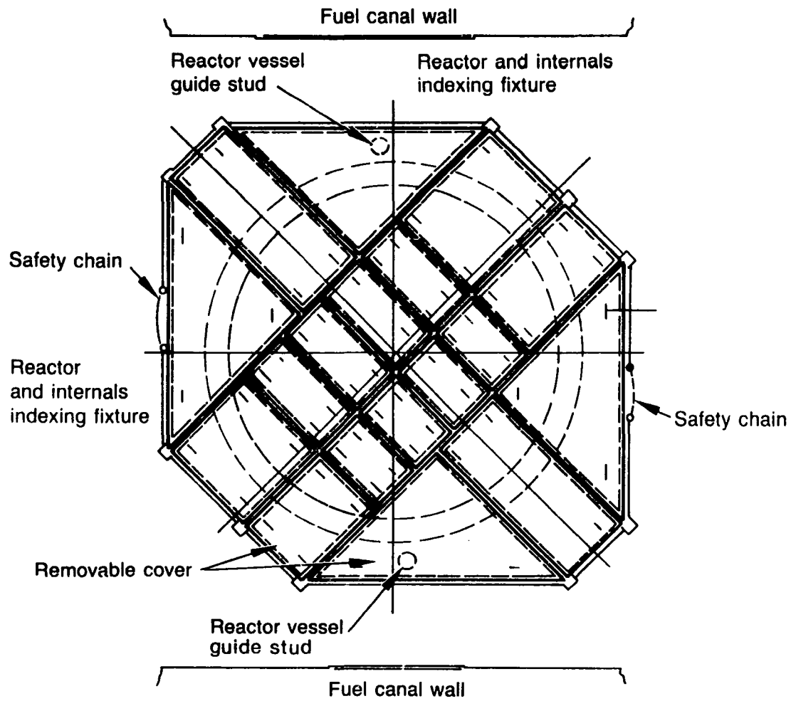
Figure A-11. IIF cover.
