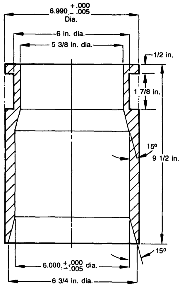
Figure A-17. Modified IIF guide bushing--normal.
